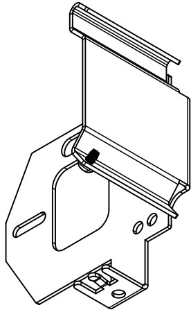
ISOMETRIC VIEW
