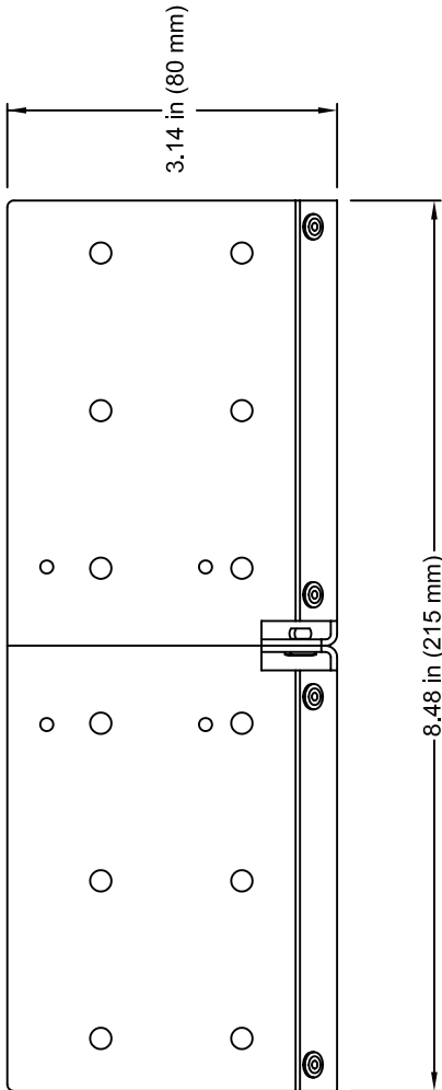
TOP VIEW
