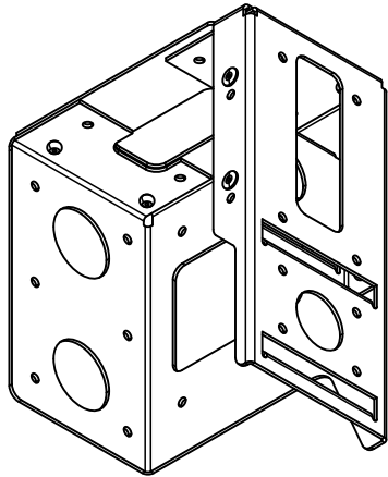
ISOMETRIC VIEW
