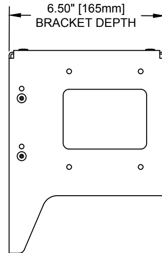
ELEVATION VIEW
