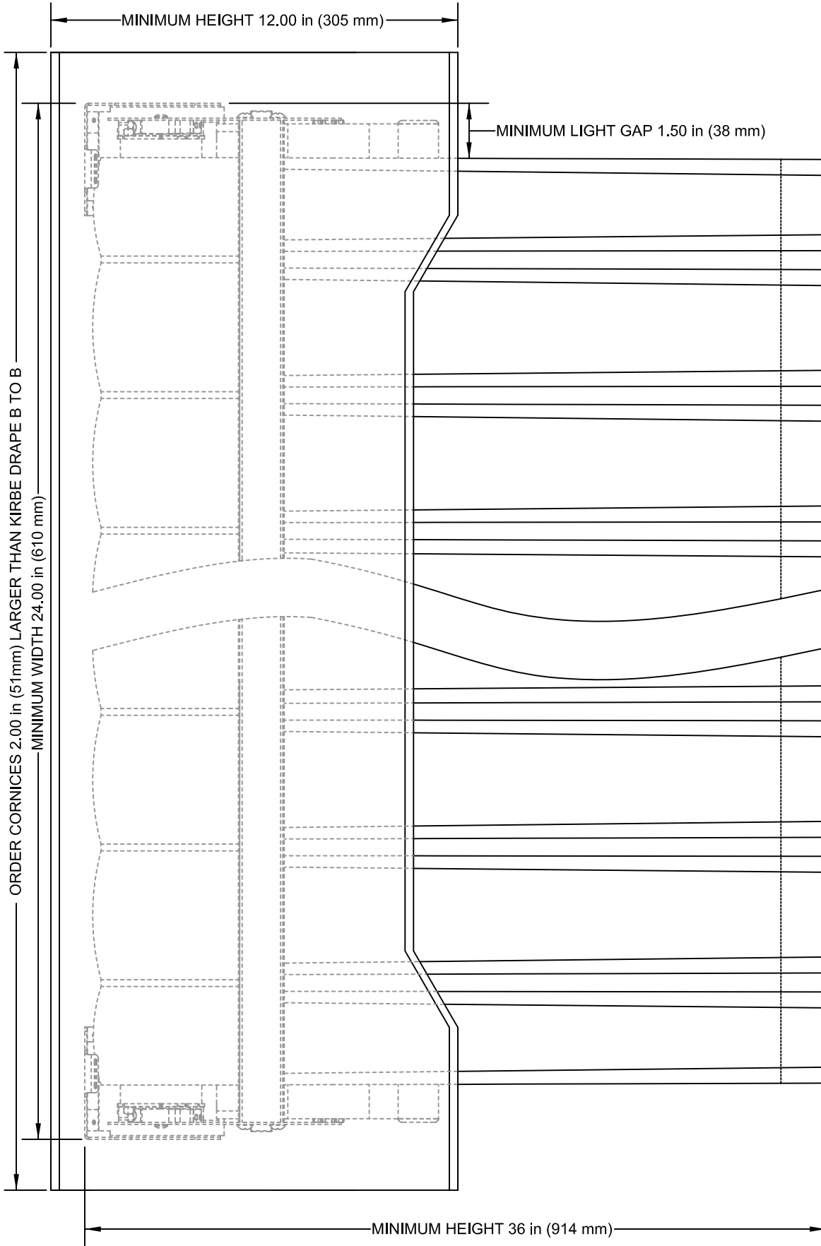
TYPICAL ELEVATION (ROOM VIEW)
