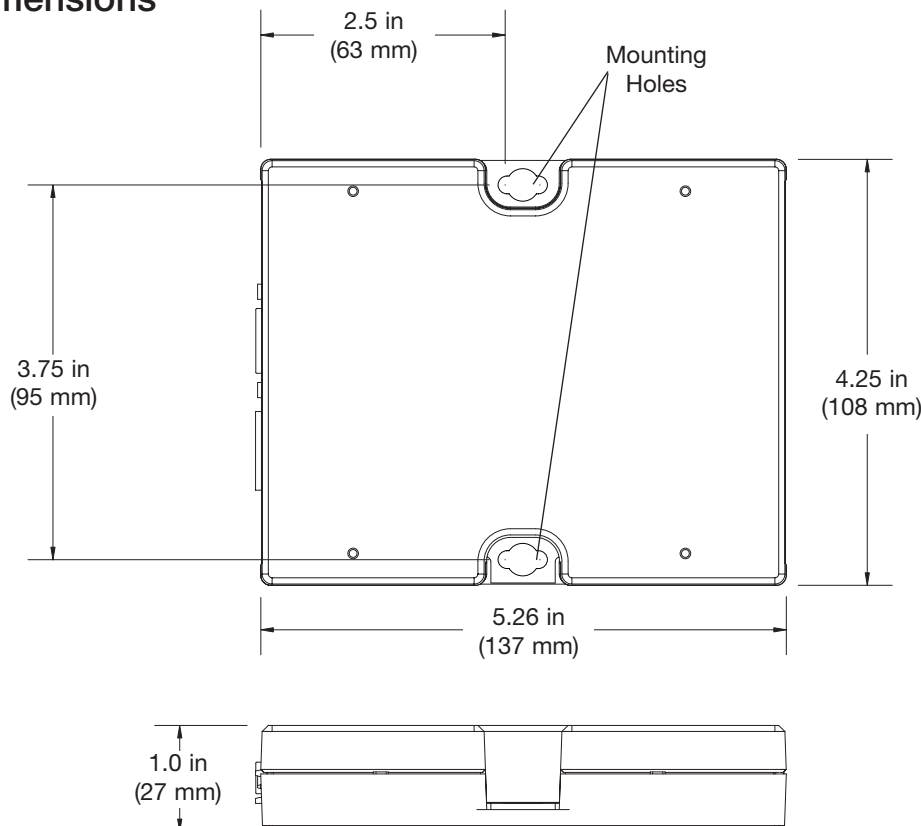
Mounting Hole Detail
