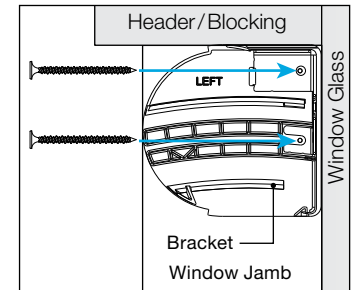
Type B Bracket
