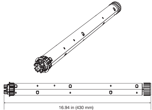
Sivoia QS roller 64 Electronic Drive Unit QSSC-EDU-10, QSSC-EDU-R64-XX
