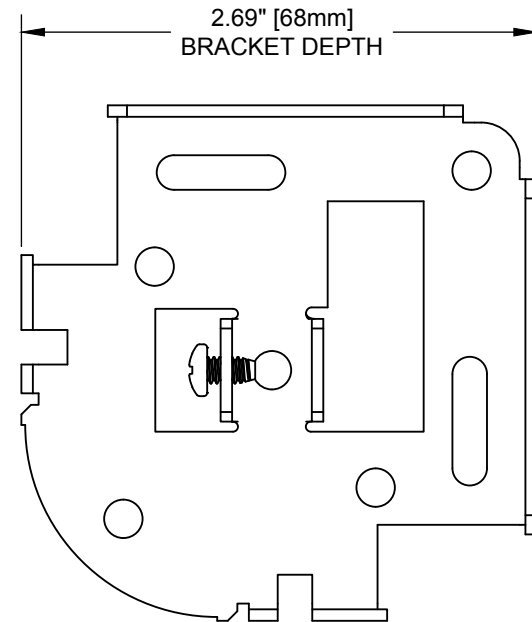
ELEVATION VIEW
