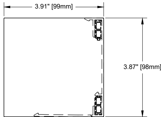
SECTION VIEW
