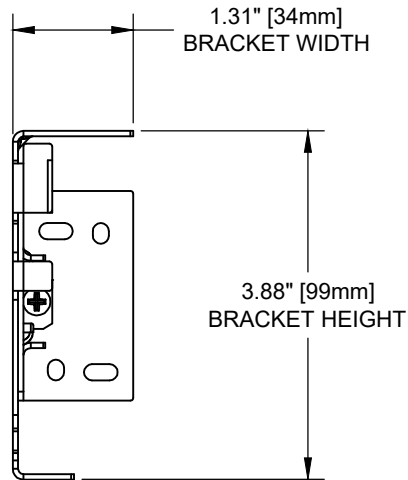
ELEVATION VIEW
