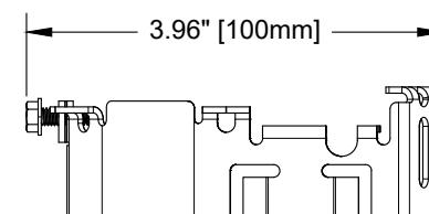
ELEVATION VIEW
