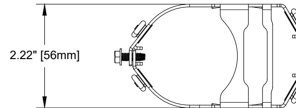
PLAN VIEW
