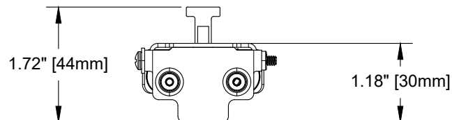
SECTION VIEW
