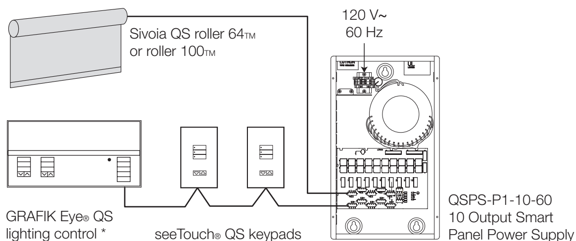
Figure D – One line diagram showing integration between a simple Sivoia QS shading system and Lutron lighting controls.
