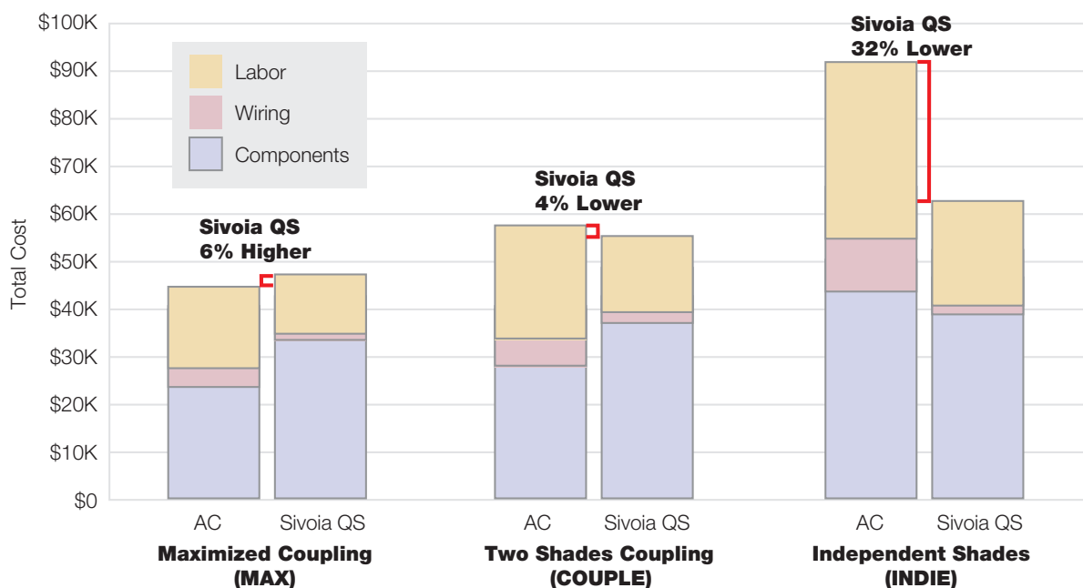
Figure A – Comparison of cost aspects for the line voltage AC and low voltage Sivoia QS shading systems
