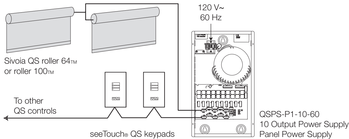
Figure C – Wiring diagram showing two drives daisy chained from one power output
