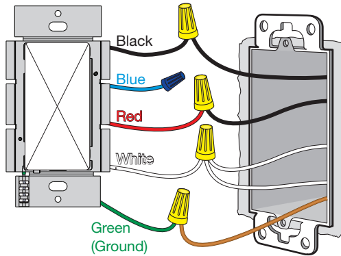
Image #32 — Dimmer with One Black Wire, One Red Wire, One Blue Wire, and one White Wire in a Single Pole Application
