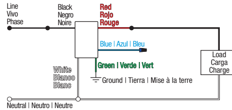
Image #32 — Dimmer with One Black Wire, One Red Wire, One Blue Wire, and one White Wire in a Single Pole Application
