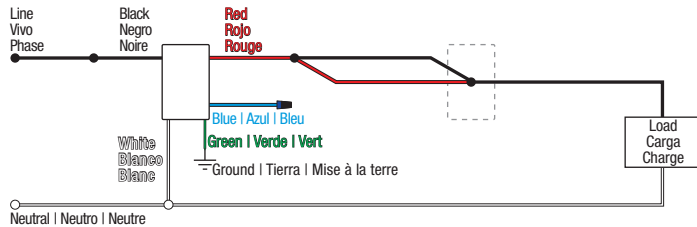
Image #33 — Dimmer with One Black Wire, One Red Wire, One Blue Wire, and one White Wire in a 3-Way Application with a Pico Remote (continued)
