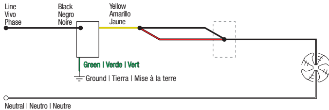
Image #78 — Fan Control with One Black Screw, One Yellow Wire and One White Wire in a 3-Way Application with a Pico Remote (continued)
