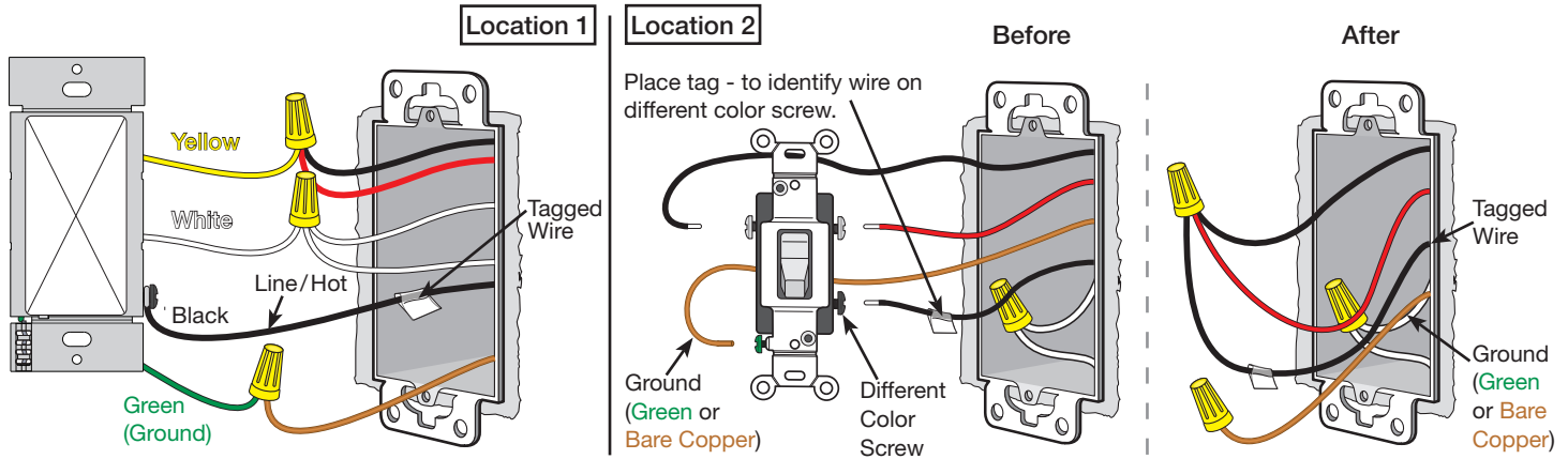
Image #78 — Fan Control with One Black Screw, One Yellow Wire and One White Wire in a 3-Way Application with a Pico Remote
