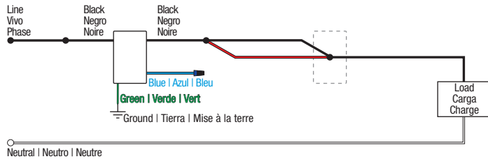
Image #12 — Caséta Switch with Two Black Wires and One Blue Wire in a 3-Way Application with a Pico Remote (continued)
