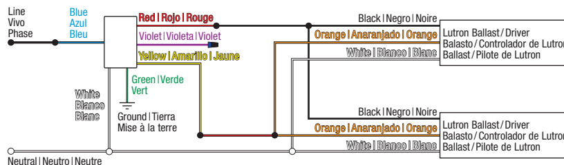
Image #42 — Dimmer with One Blue Wire, One Violet Wire, One Red Wire, One Yellow Wire and One White Wire in a Single Pole Application
