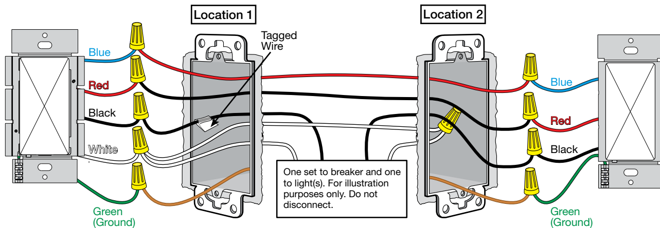
Image #86 — Caséta Claro Smart Switch with One Black, One Red, One Blue, and One White wire in a 3-Way Application with a Companion Control
