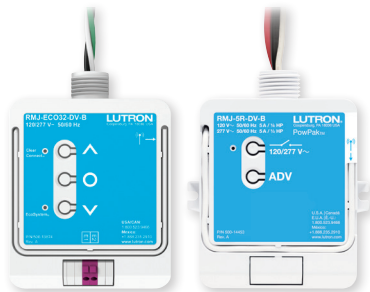
Junction Box Mount Dimmers and Switches
