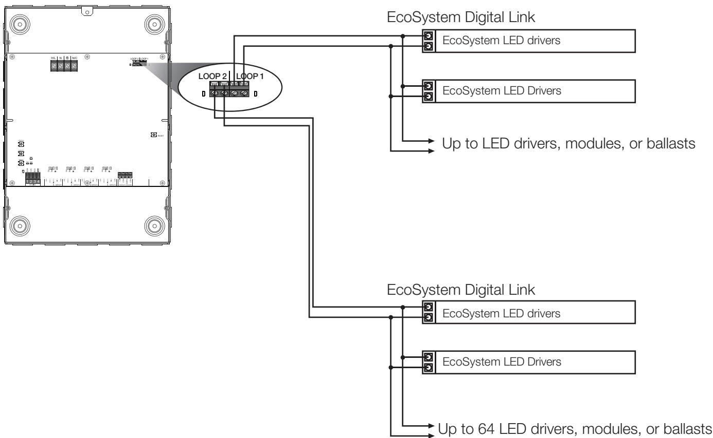
Energi Savr Node unit with EcoSystem
