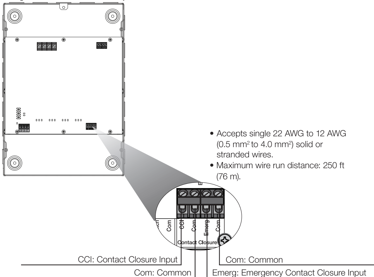
Energi Savr Node unit with EcoSystem
