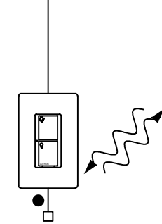
PD-5WS-DV-WH 120/277V~, 50/60 Hz CASETA ORIGINAL IN-WALL SWITCH 2 BUTTON CONTROL SHOWN WITH CW-1-WH CLARO WALLPLATE (1 GANG US BACKBOX BY OTHERS) LOCATION TBD
