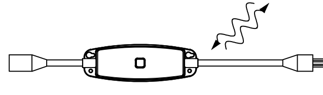
PD-15OUT-BL 120V~, 50/60 Hz CASETA OUTDOOR SMART PLUG SWITCHES 15A / 0.5HP / 1200 VA MAX EXTERIOR-RATED (IP65) 6.875"(H) X 2.25"(W) X 1.5"(D) (175mm X 57mm X 38mm) RECEPTACLE CORD LENGTH: 5.125" (130mm) PLUG CORD LENGTH: 7" (178mm) LOCATION TBD
