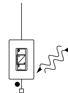
PD-6WCL-WH 120V~, 50/60 Hz CASETA ORIGINAL IN-WALL DIMMER LED, CFL, INC. & HAL LOADS 2 BUTTON CONTROL WITH RAISE/LOWER SHOWN WITH CW-1-WH CLARO WALLPLATE (1 GANG US BACKBOX BY OTHERS) LOCATION TBD
