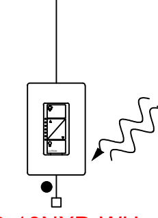
PD-10NXD-WH 120V~, 50/60 Hz CASETA ORIGINAL IN-WALL PRO DIMMER LED, CFL, INC. & HAL LOADS 2 BUTTON CONTROL W/ RAISE/LOWER SHOWN WITH CW-1-WH CLARO WALLPLATE (1 GANG US BACKBOX BY OTHERS) LOCATION TBD
