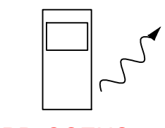
PD-OSENS CASETA OCCUPANCY/VACANCY SENSOR 180° COVERAGE 4.35"[110mm] (H) X 1.8"[46mm] (W) X 1.35"[34mm] (D) *DEVICE CAN BE WALL-MOUNTED AND IS BATTERY POWERED (POWER FEED NOT REQUIRED) LOCATION TBD
