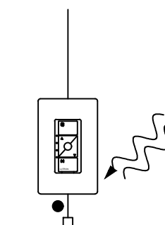
PD-FSQN-WH 120V~, 50/60 Hz CASETA ORIGINAL FAN SPEED CONTROL 3 BUTTON CONTROL W/ RAISE/LOWER SHOWN WITH CW-1-WH CLARO WALLPLATE (1 GANG US BACKBOX BY OTHERS) LOCATION TBD
