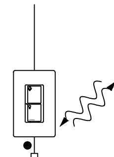
PD-6ANS-WH 120V~, 50/60 Hz CASETA ORIGINAL IN-WALL SWITCH NEUTRAL WIRE REQUIRED 2 BUTTON CONTROL SHOWN WITH CW-1-WH CLARO WALLPLATE (1 GANG US BACKBOX BY OTHERS) LOCATION TBD
