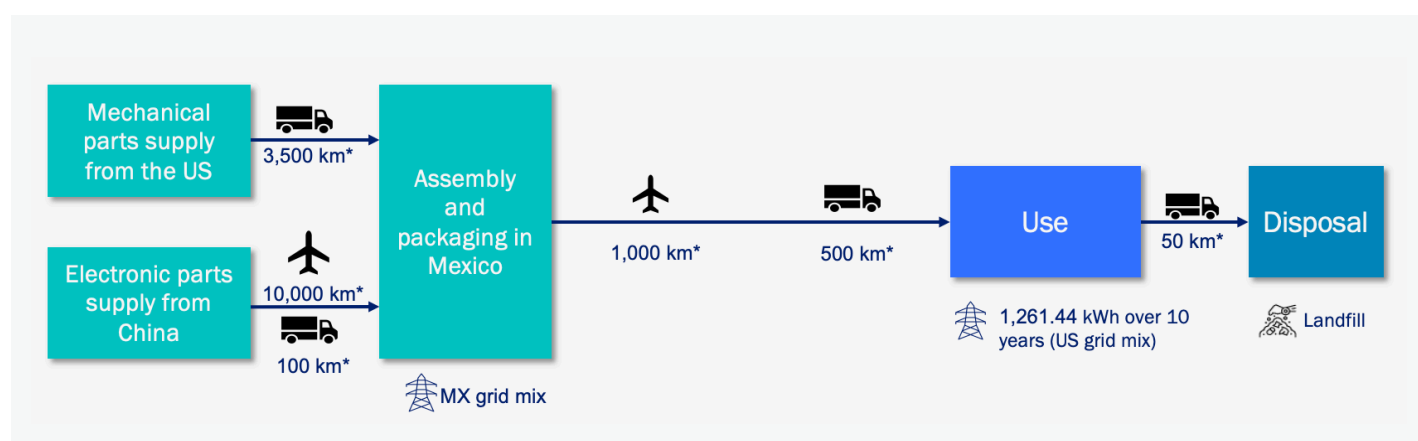
Figure 2: Schematic representation of the QSN-2DAL-UNV-D's life cycle (*Default transportation scenario for continental, intercontinental and domestic transportation)
