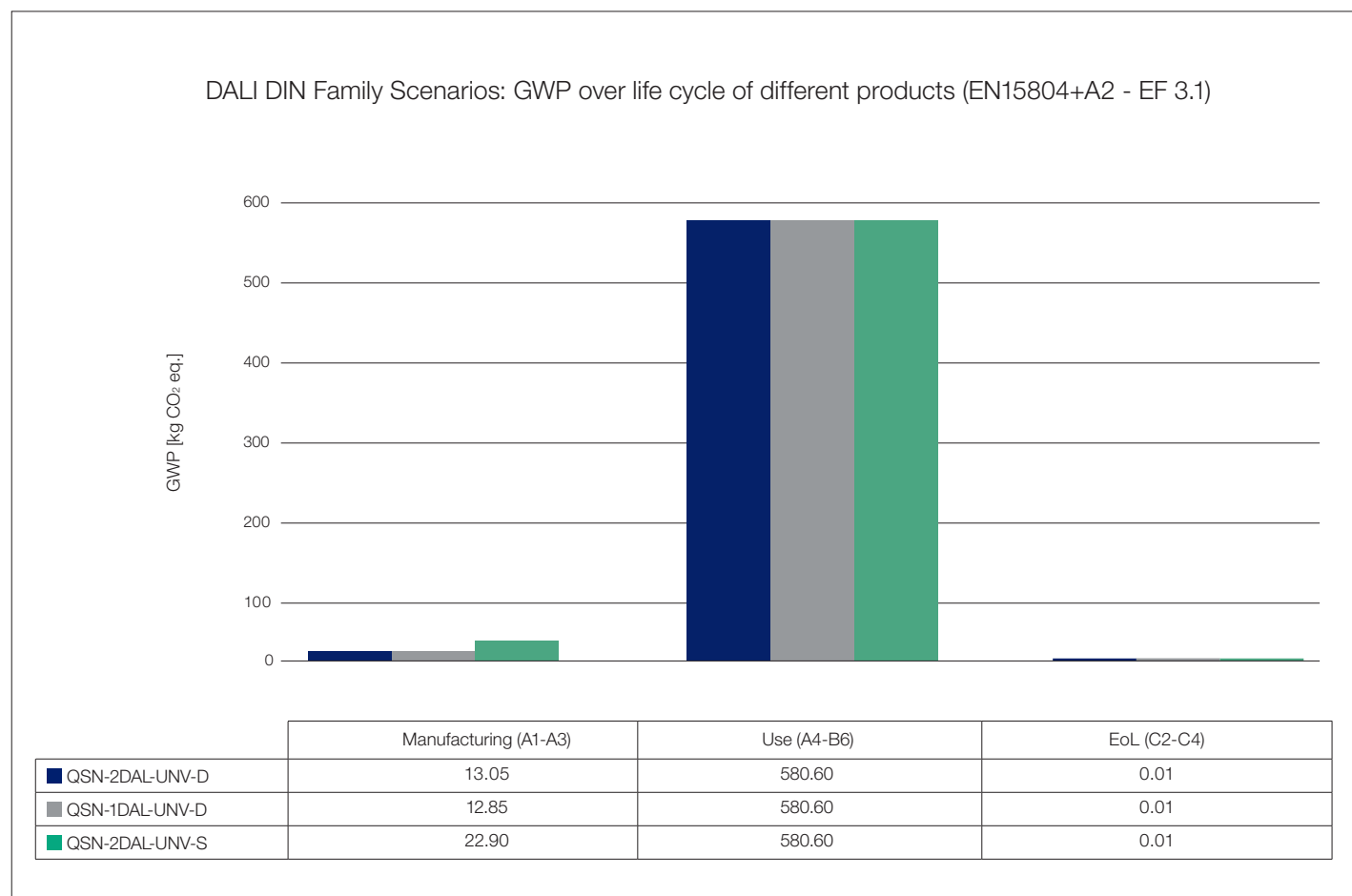
Figure 6: Climate Change potential in the Life Cycle of different DIN Module Controller DALI variants
