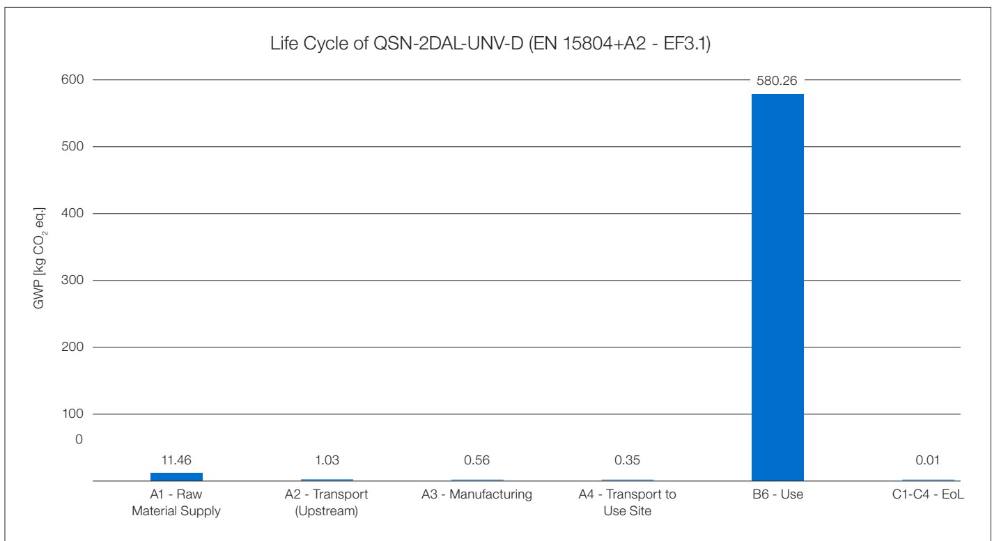
Figure 3: Climate Change Potential of one unit of DIN Module Controller
