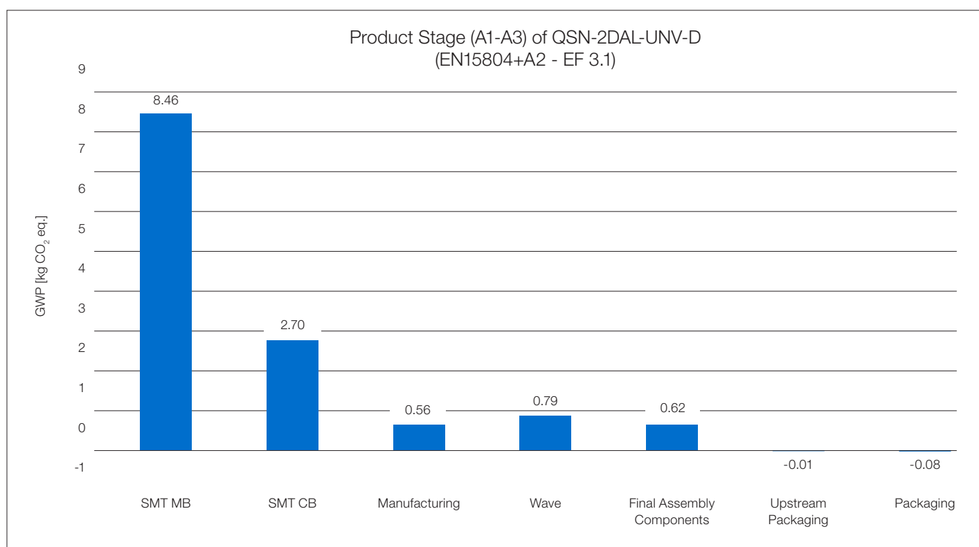
Figure 4: Climate Change Potential in the Manufacturing Stage of one unit of DIN Module Controller
