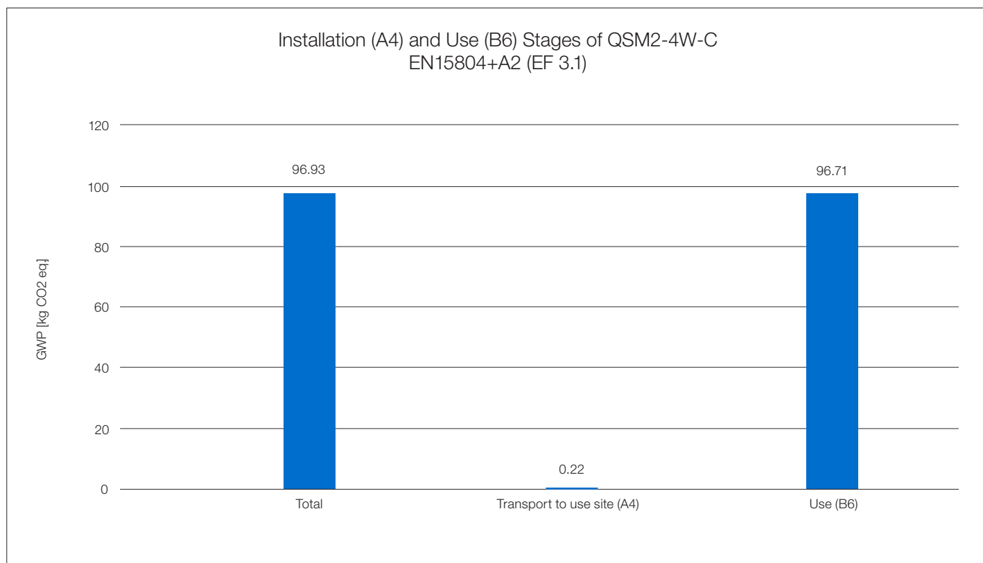
Figure 5: Climate Change Potential in the Installation and Use Stages of one unit of QS Sensor Module
