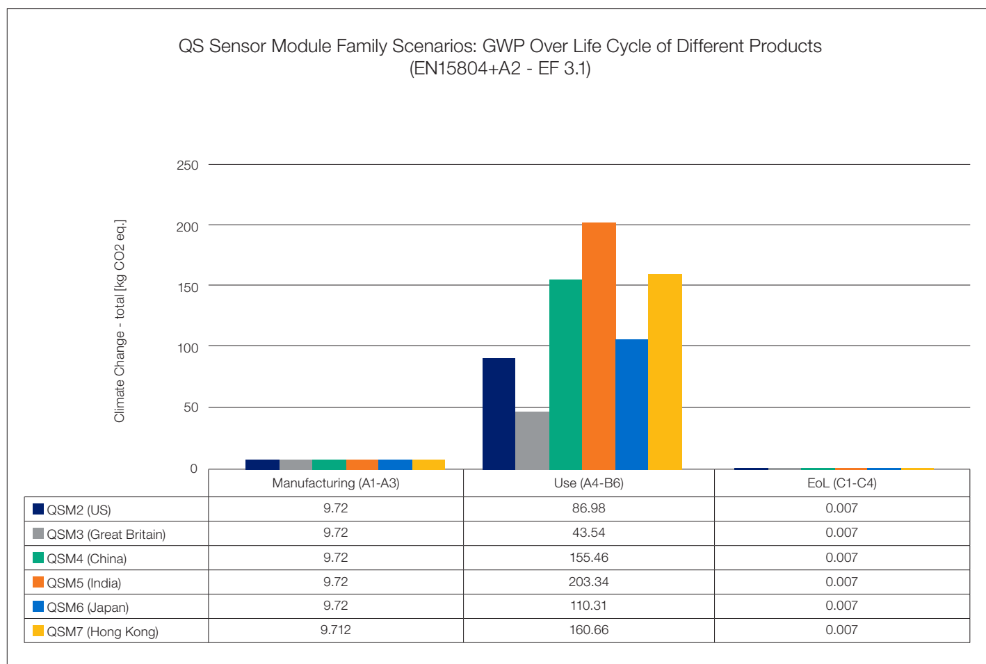
Figure 6: Climate Change potential in the Life Cycle of different QS Sensor Module variants
