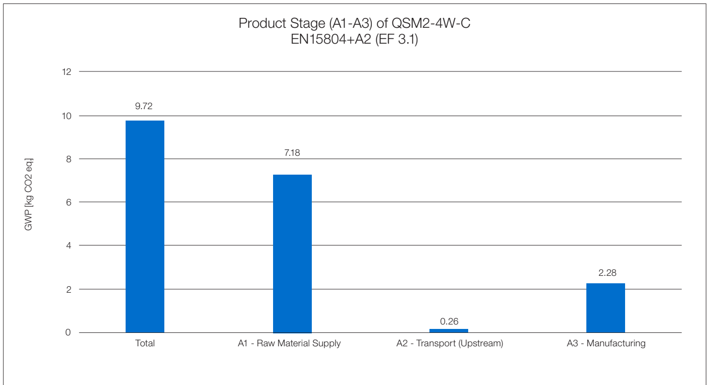
Figure 4: Climate Change Potential in the Manufacturing Stage of one unit of QS Sensor Module
