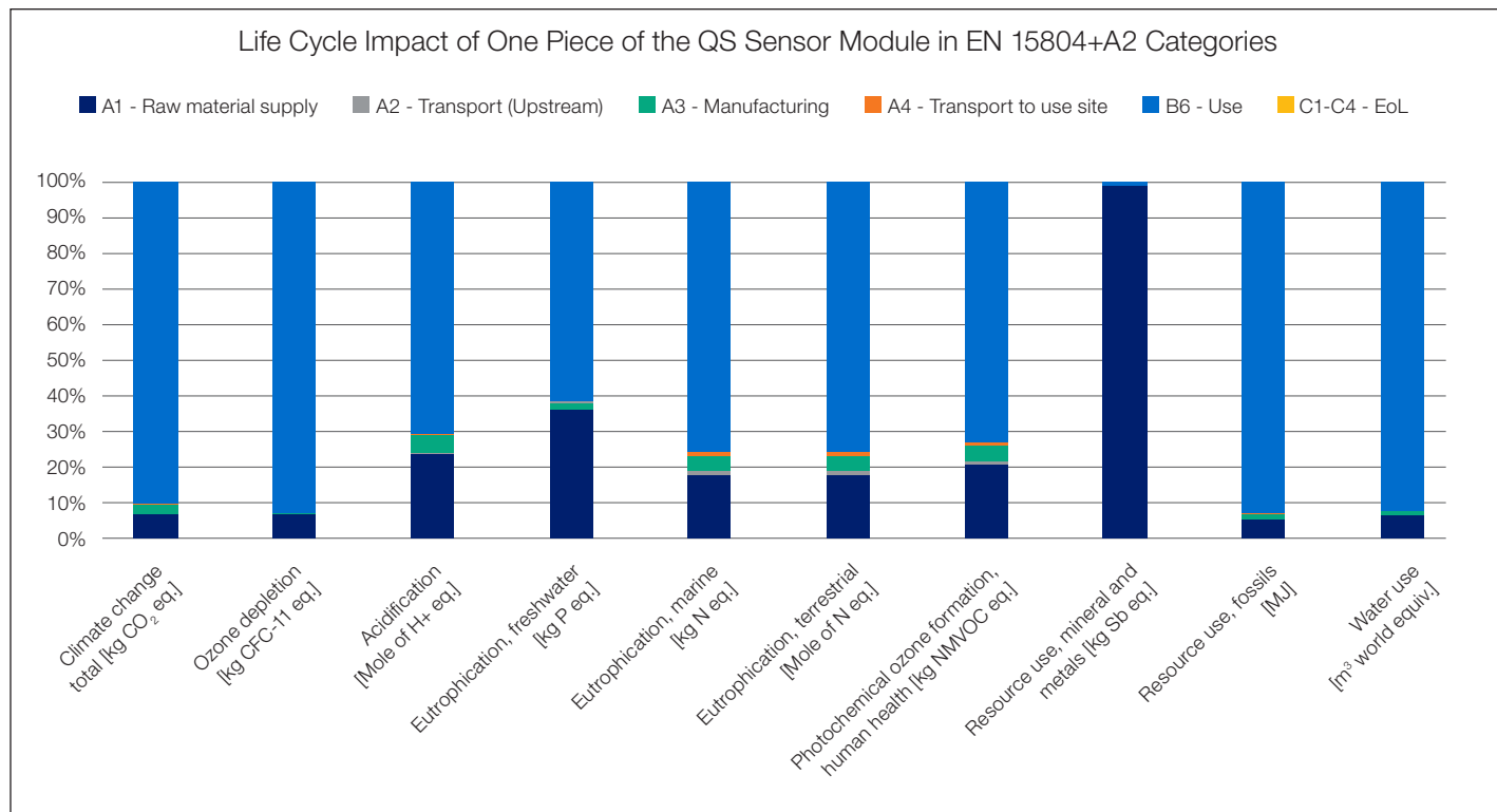
Figure 7: Life Cycle Impact of one piece of the QS Sensor Module in EN 15804+A2 categories
