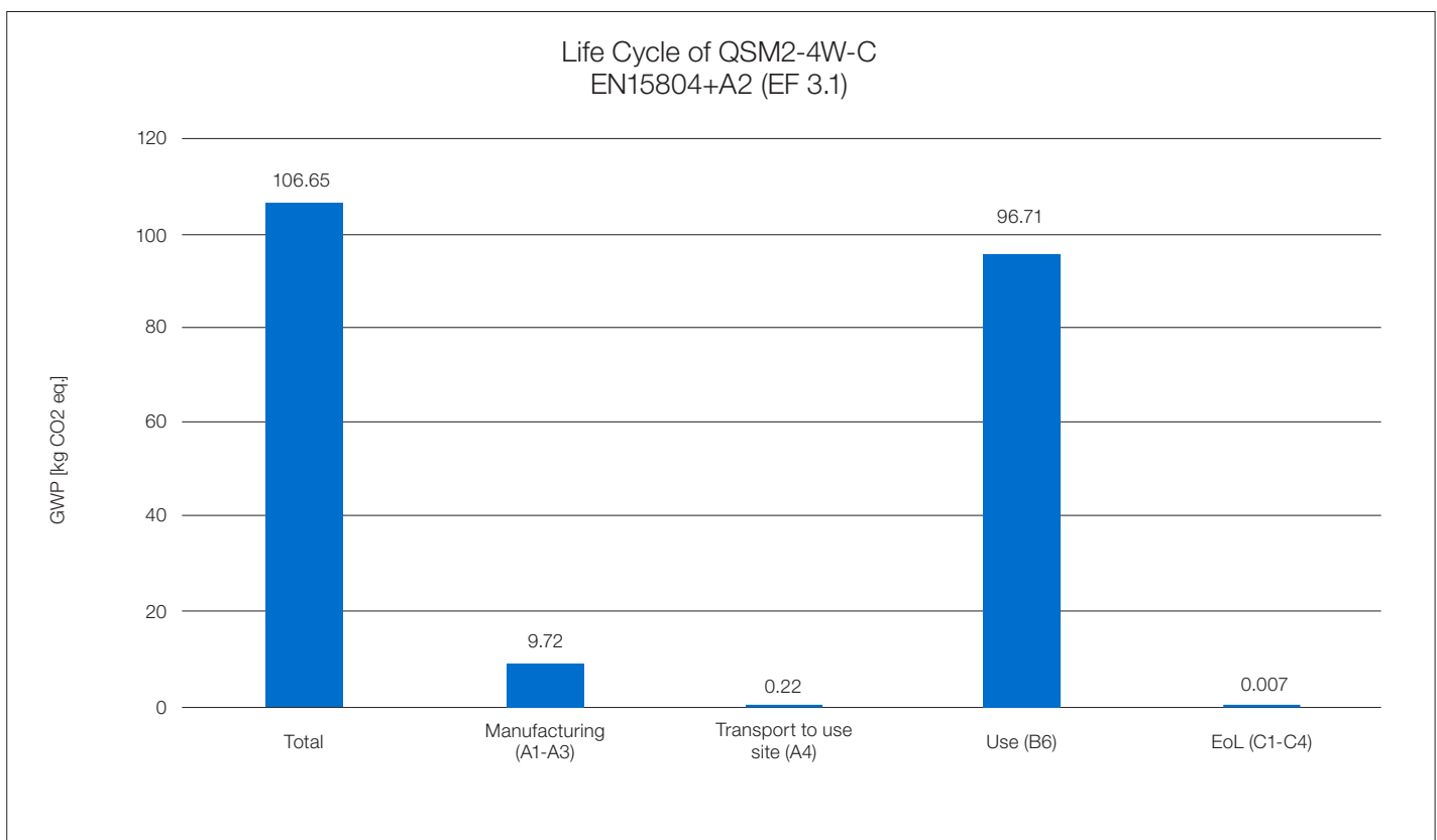
Figure 3: Climate Change Potential of one unit of QS Sensor Module
