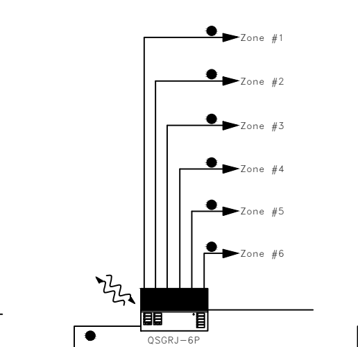
QSGRJ-6P + 2 Shades
