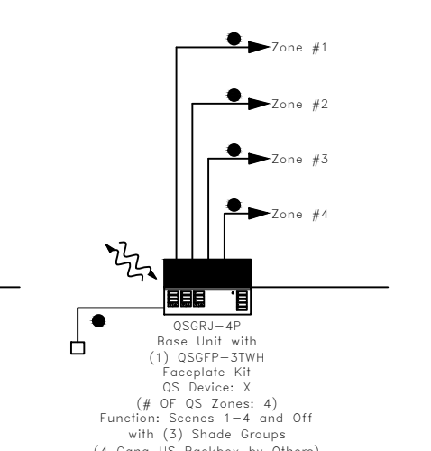
QSGRJ-4P + 3 Shades
