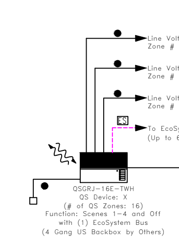
QSGRJ-16E-TWH
