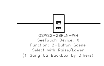
QSW2-2BRLN
