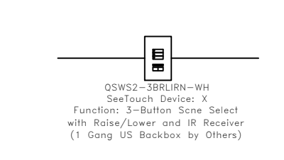
QSW2-3BRLIRN
