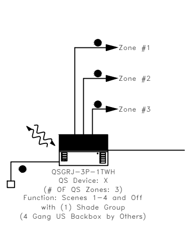
QSGRJ-3P-1TWH
