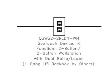
QSW2-2RLDN
