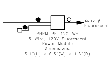
PHPM-3F-120
