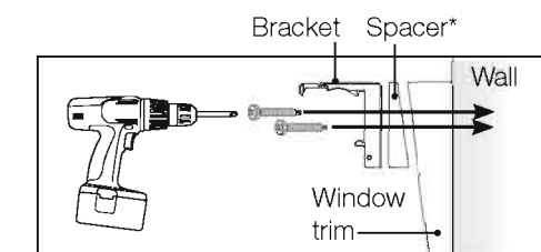
Side view *Optional (not included)
